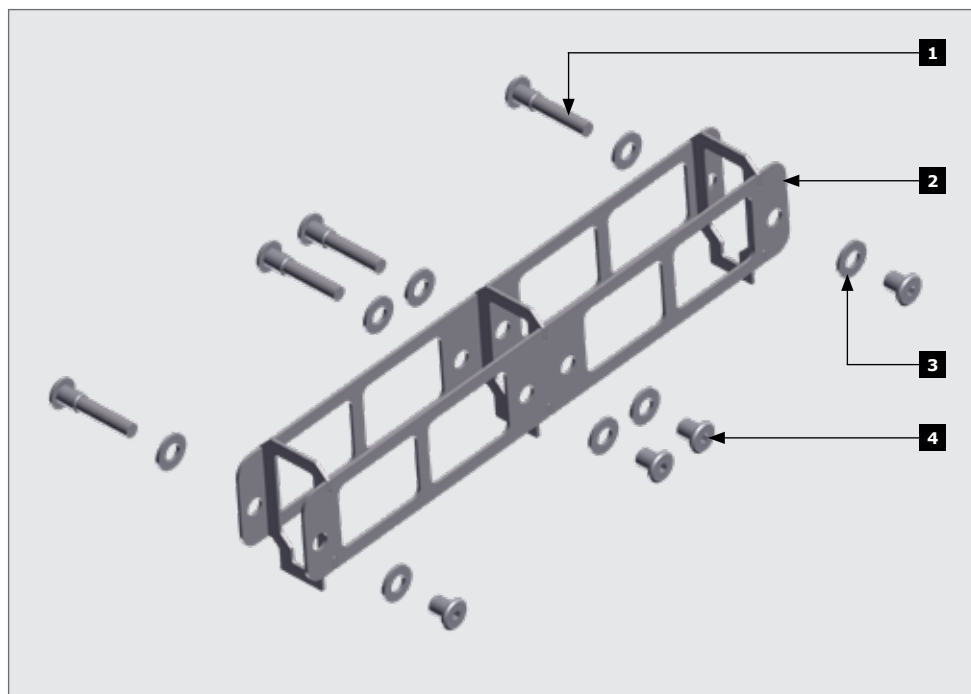
FIGURE 2. PRODUCT IDENTIFICATION - HARDWARE
